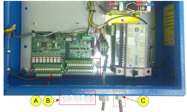
Figure 5-31: Control Module Interior Generic
