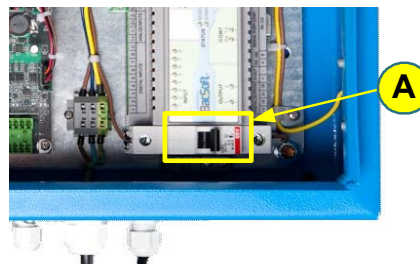
Figure 6-1: Control Module
