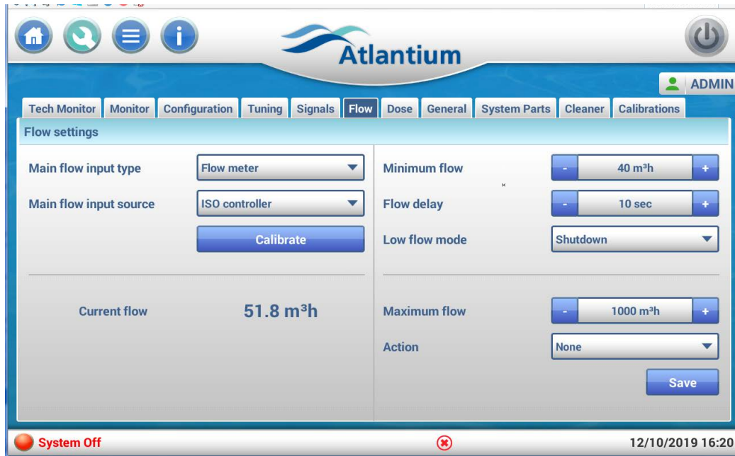
Figure 7-10: Flow Setting Screen – Flow Meter
