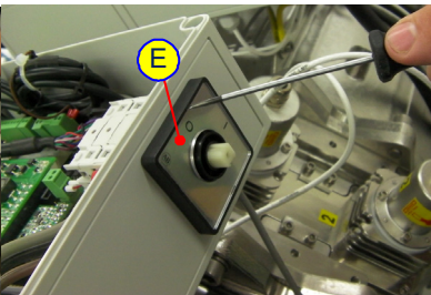
Figure 5-39: Replacing the Power Cable 2
