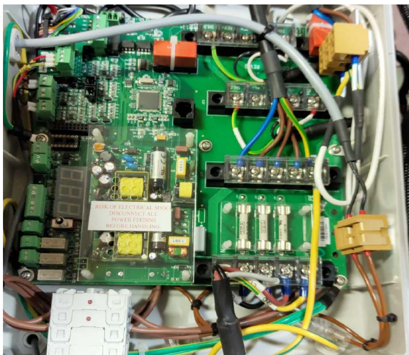
Figure 5-22: Connection Box with LM Card 700/750 (for system with ultrasonic cleaner)
