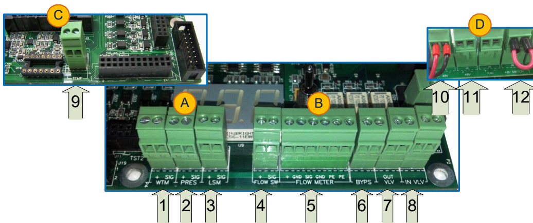
Figure 5-29: Connectors on Connection Box Card 1300+1400
