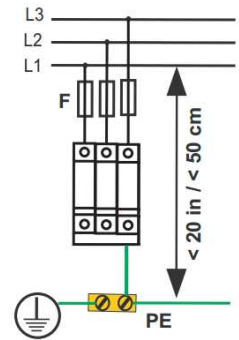
Figure 5-14: Surge protection device wiring - 440/480VAC
