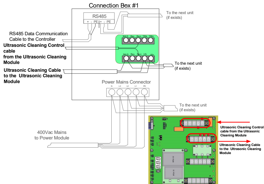
Figure 5-24: Cabling Schematic Diagram
