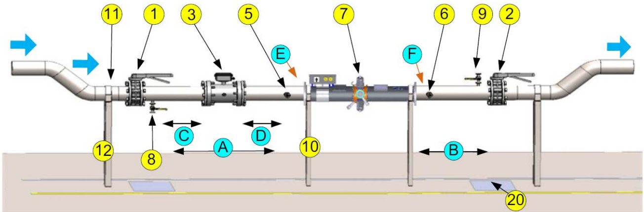
Figure 3-1: Generalized Atlantium system setup, horizontal (no bypass)
