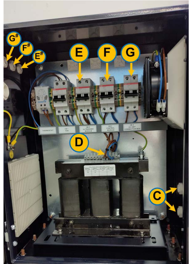
Figure 5-28: Power Module - connections
