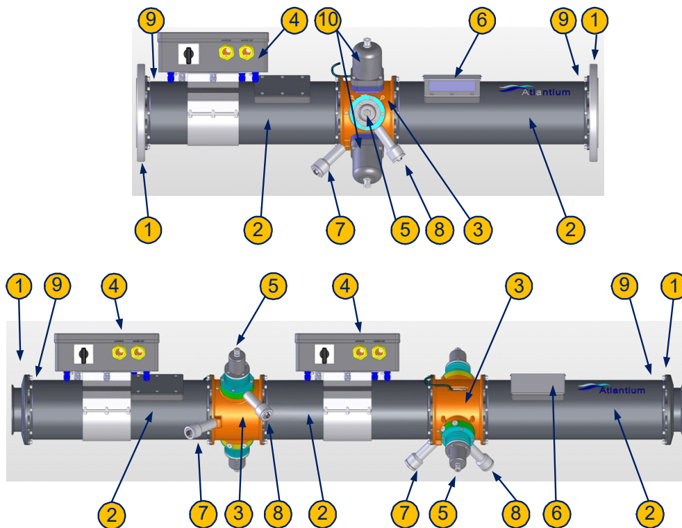
Figure 2-1: RZ104-11 (top) with ultrasonic cleaner, RZ104-12 (bottom) without a cleaner.
