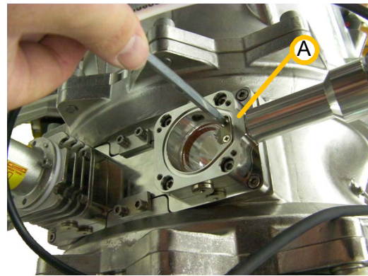
Figure 10-18: (Generic) Cleaning the UV Intensity Sensor's Mirror
