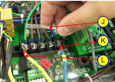
Figure 5-42: Replacing the Power Cable 5
