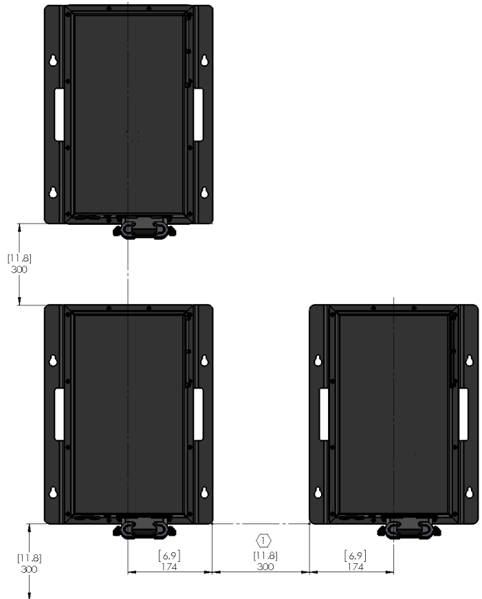
Figure 5-18: Multiple Ballast Module C Installation Diagram
