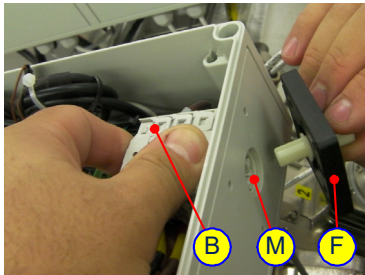
Figure 5-43: Replacing the Power Cable 6
