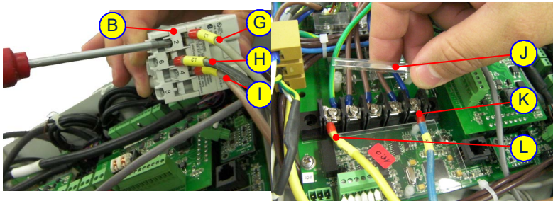
Figure 5-41: Replacing the Power Cable 4
